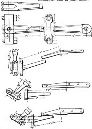
Figs. 255-263. Boiler Braces. Atlantic (4-4-2) Locomotive with Belpaire Boiler. P. R. R.
